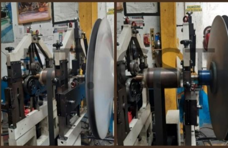
REPAIR MOTOR (BALANCING IMPELER)
